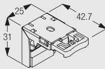
10101 Bracket
